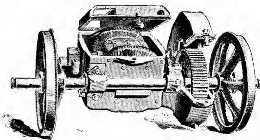
Fig. 5678. MOTOR ATTACHED TO A PAIR OF WHEELS, WITH CASE OPEN TO SHOW ATTACHMENT.
